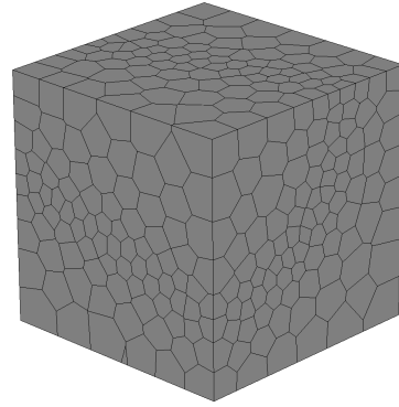
(a) Voronoi diagram slice at x = 0 .
