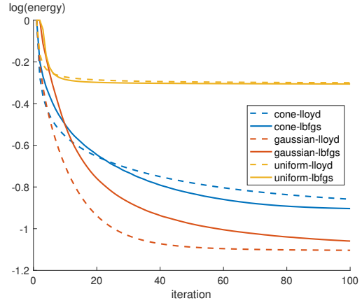
(a) Energy (Eq. 3 versus iteration.
