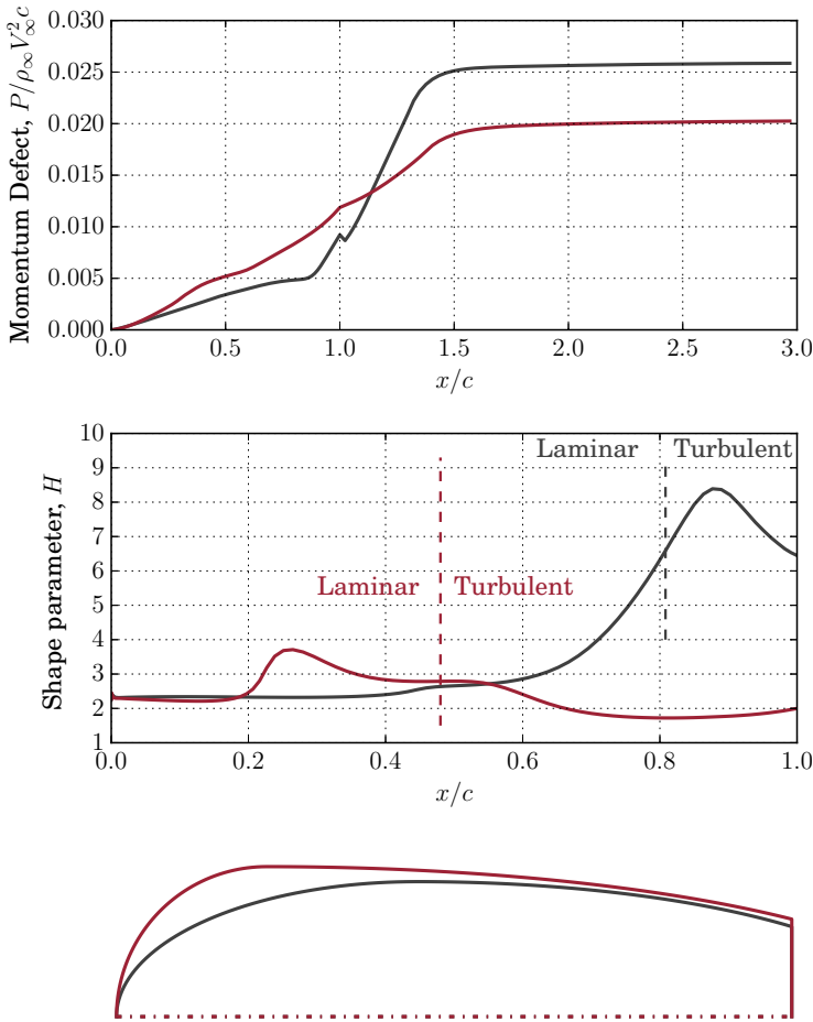
Figure 7. Shape parameter and momentum defect for different dummy positions. The shape in gray positions the dummy in the middle resulting in a flatter shape ( C_{DA} = 0.0553 ), the shape in red positions the dummy in the nose ( C_{DA} = 0.0431 ).
