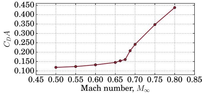
Figure 14. C_{DA} as a function of Mach number for the final design. The large drag build-up starts around M_\infty = 0.675 . Note that the freestream density is kept constant, therefore the Reynolds number increases proportionally with Mach number.
